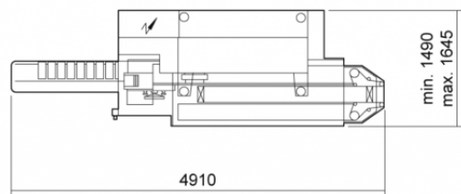
MACHINE LAYOUT
